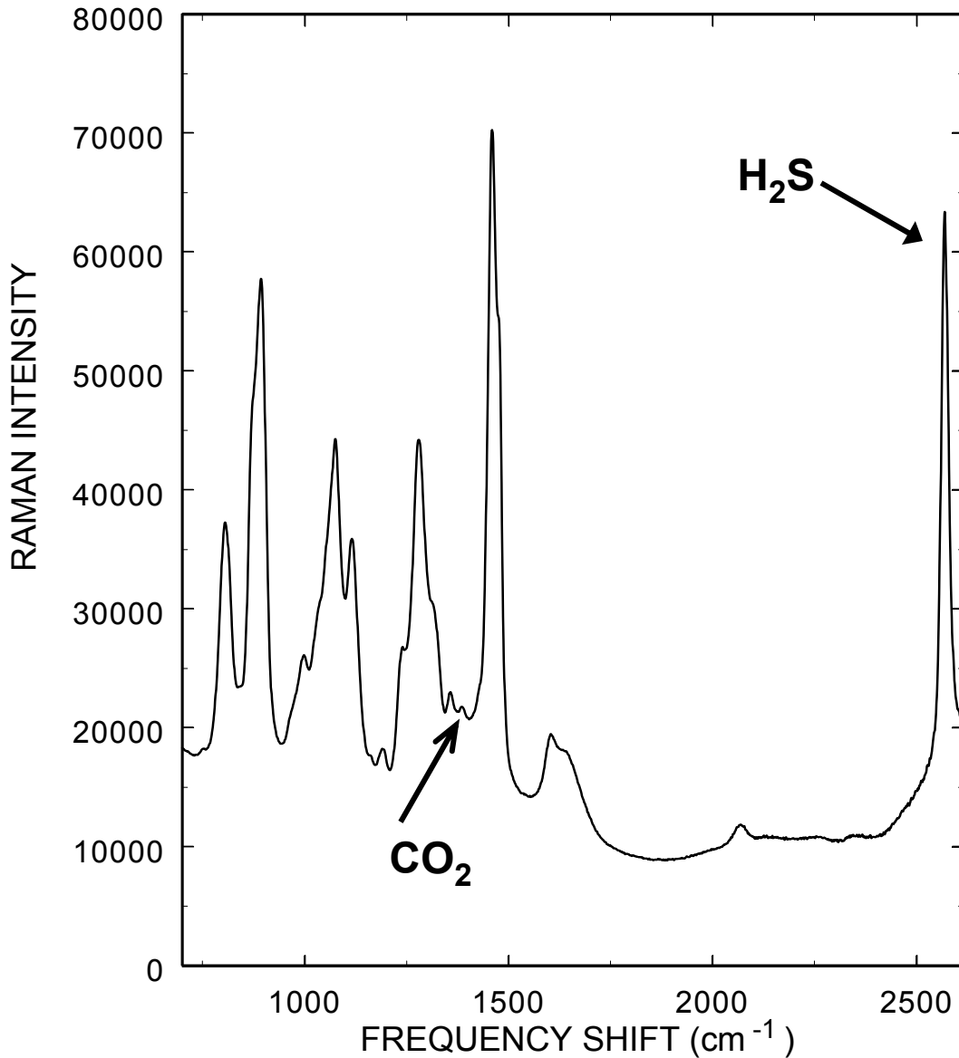
Typical spectra from amines used to remove acid gasses such as H 2 S and CO 2 .
