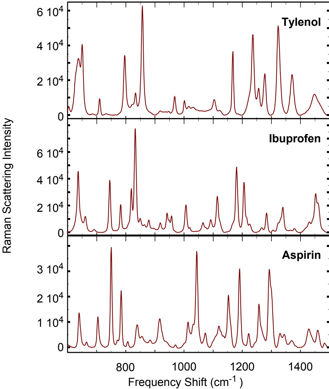
Spectra of three different common Pharmaceuticals.
